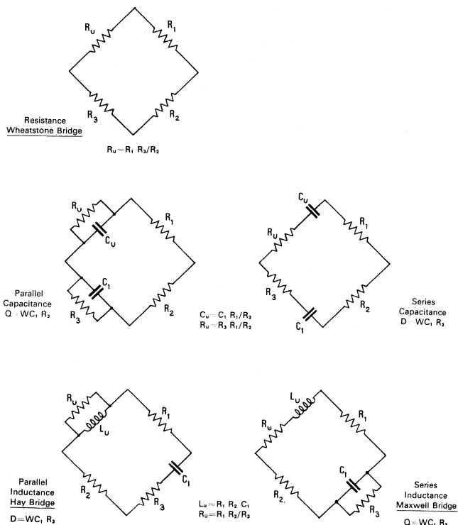
Fig. 1 Impedance-ratio-arm bridges.
