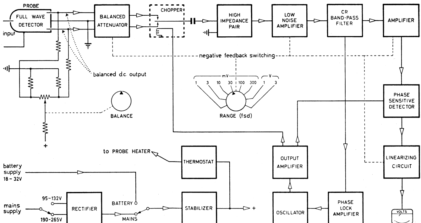
Block diagram of R.F. Electronic Millivoltmeter type TF 2603
