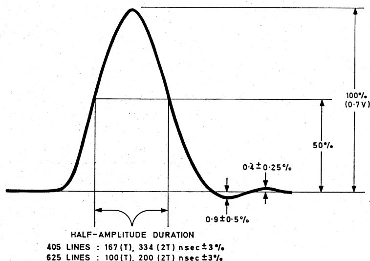
Fig. 1. Sine squared pulse showing shape and size of overshoots.
