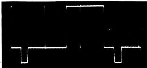
625 line Monochrome Waveform TF 2905/8
