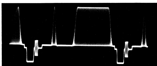
Combined Luminance Chrominance, 525 line TF 2905/9
