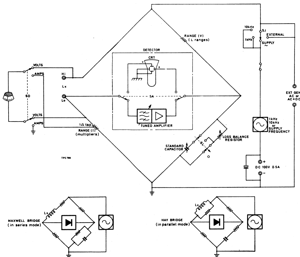
Functional diagram
