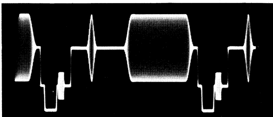
Chrominance Waveform on Pedestal, 525 line TF 2905/9
