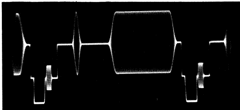
Chrominance Waveform on Pedestal, 625 line TF 2905/8
