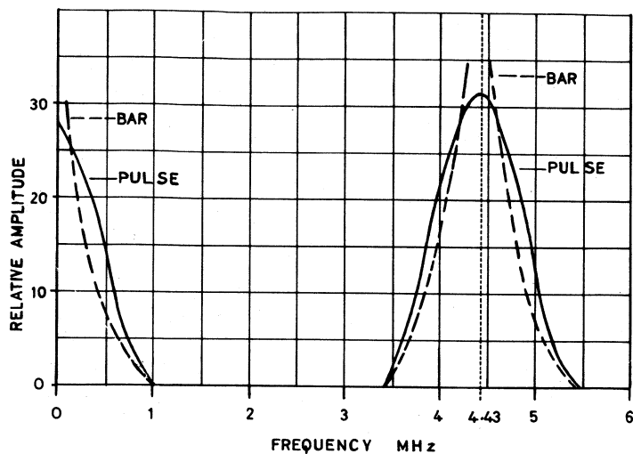
Fig. 7. Spectrum of combined luminance and chrominance sine squared pulse and bar.
