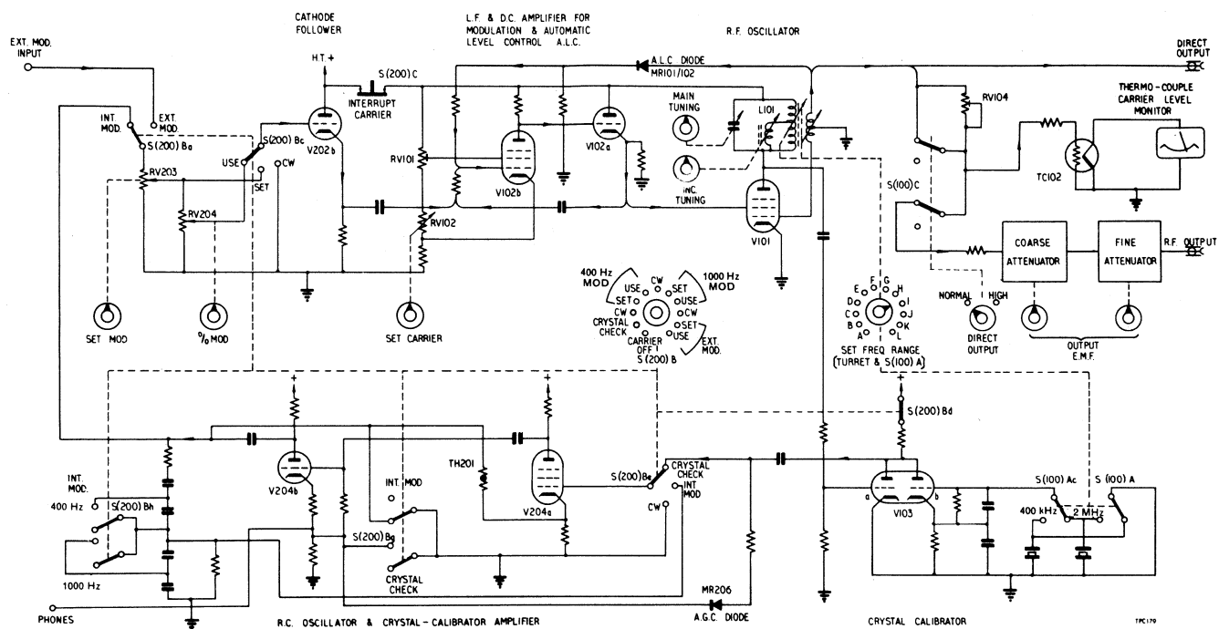
Functional Diagram of TF 144H/4
