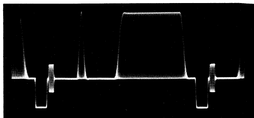
Combined Luminance and Chrominance, 625 line TF 2905/8
