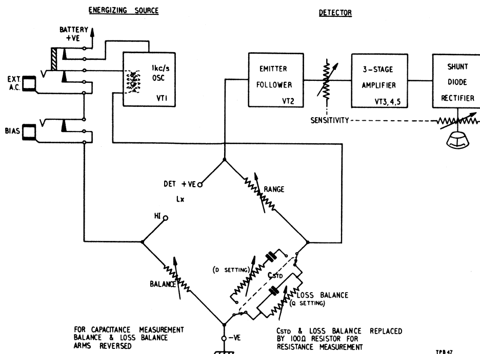
Functional Diagram for A.C. Measurements
