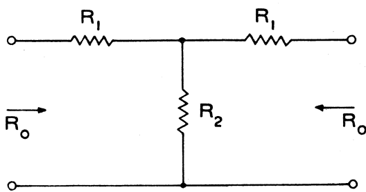
T Network
