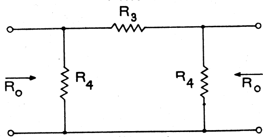
pi Network
