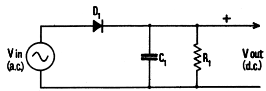
Fig. 3 Peak Detector (series configuration).
