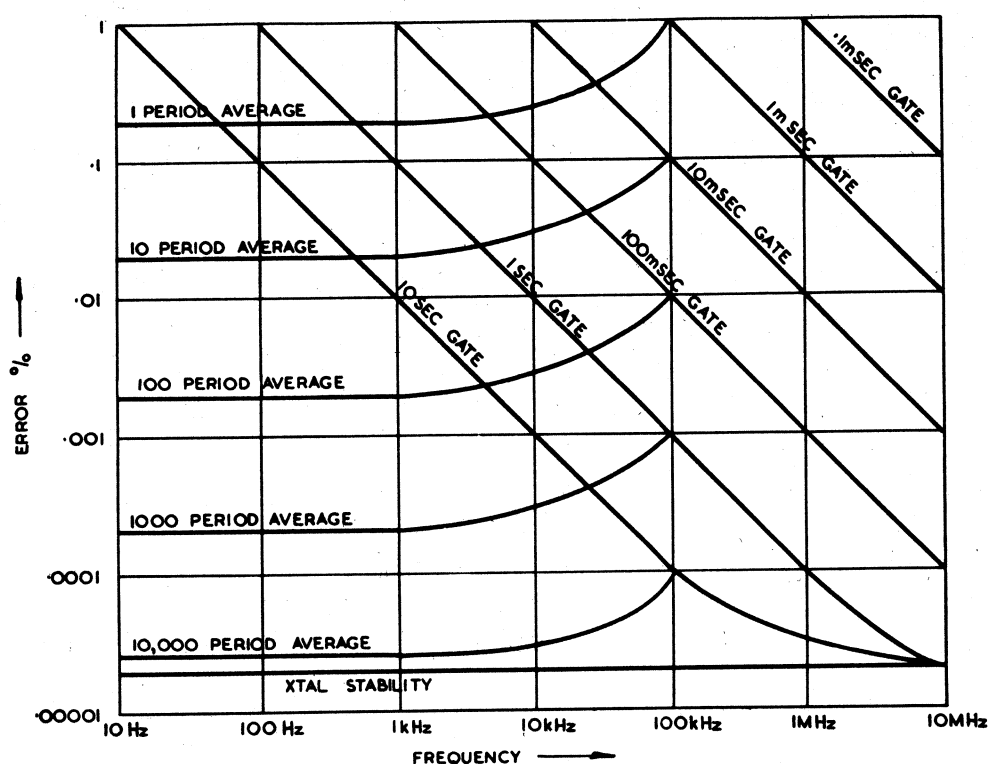
Accuracy chart
