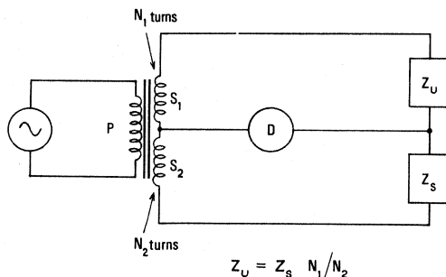
Fig. 2 Transformer-ratio-arm bridge.
