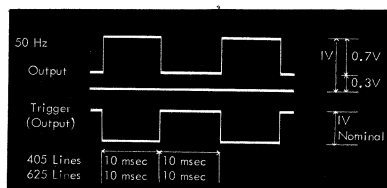
Waveform for I.f. response measurement
