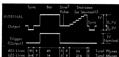
Waveform for general assessment (monochrome) with internal trigger
