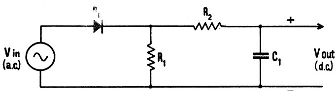
Fig. 1 Average Detector.
