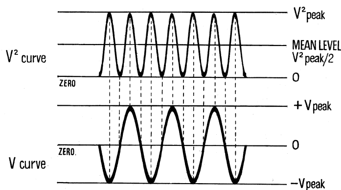
Fig. 5 Sinewave voltage and power waveforms.
